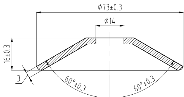
P18.5 SUS304-16mm Q'ty:01
