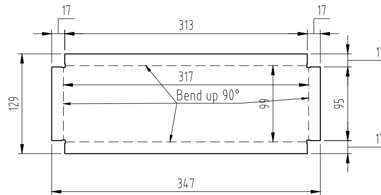
Expansion P21.1 A240 304-2mm Q'ty:32
