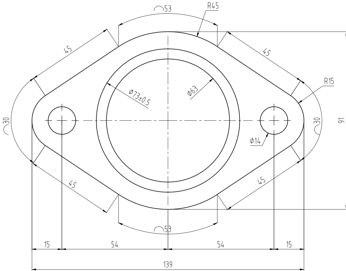
P18.1 SUS304-6mm Q'ty:2
