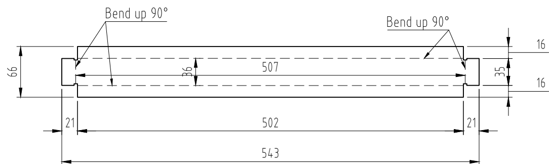
Expansion P21.2 A240 304-2mm Q'ty:128
